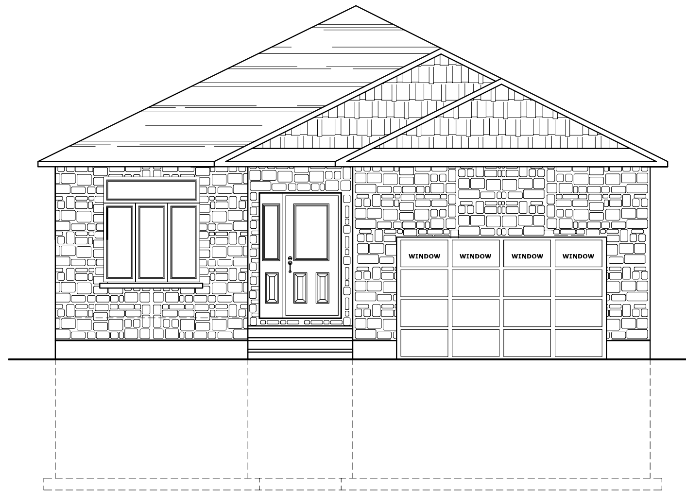
MODEL FRONT ELEVATION P2919, 1185 SQFT
