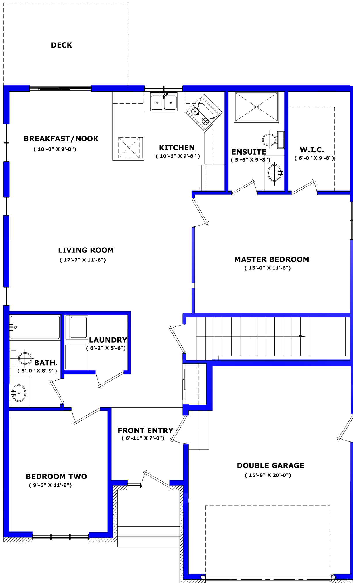
MODEL GROUND FLOOR PLAN P2919, 1185 SQFT
