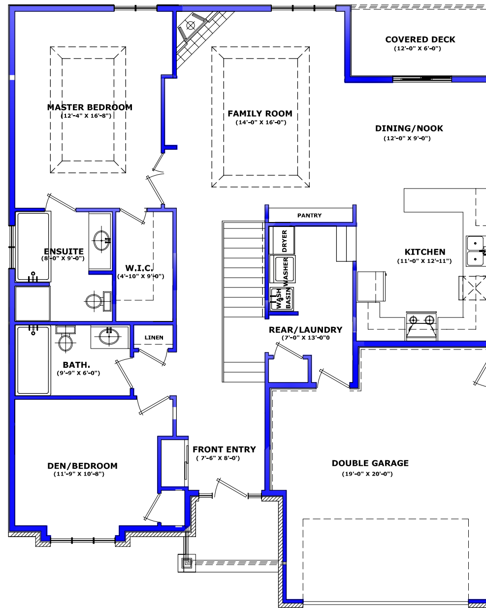
MODEL P2906 GROUND FLOOR PLAN 1461 SQFT
