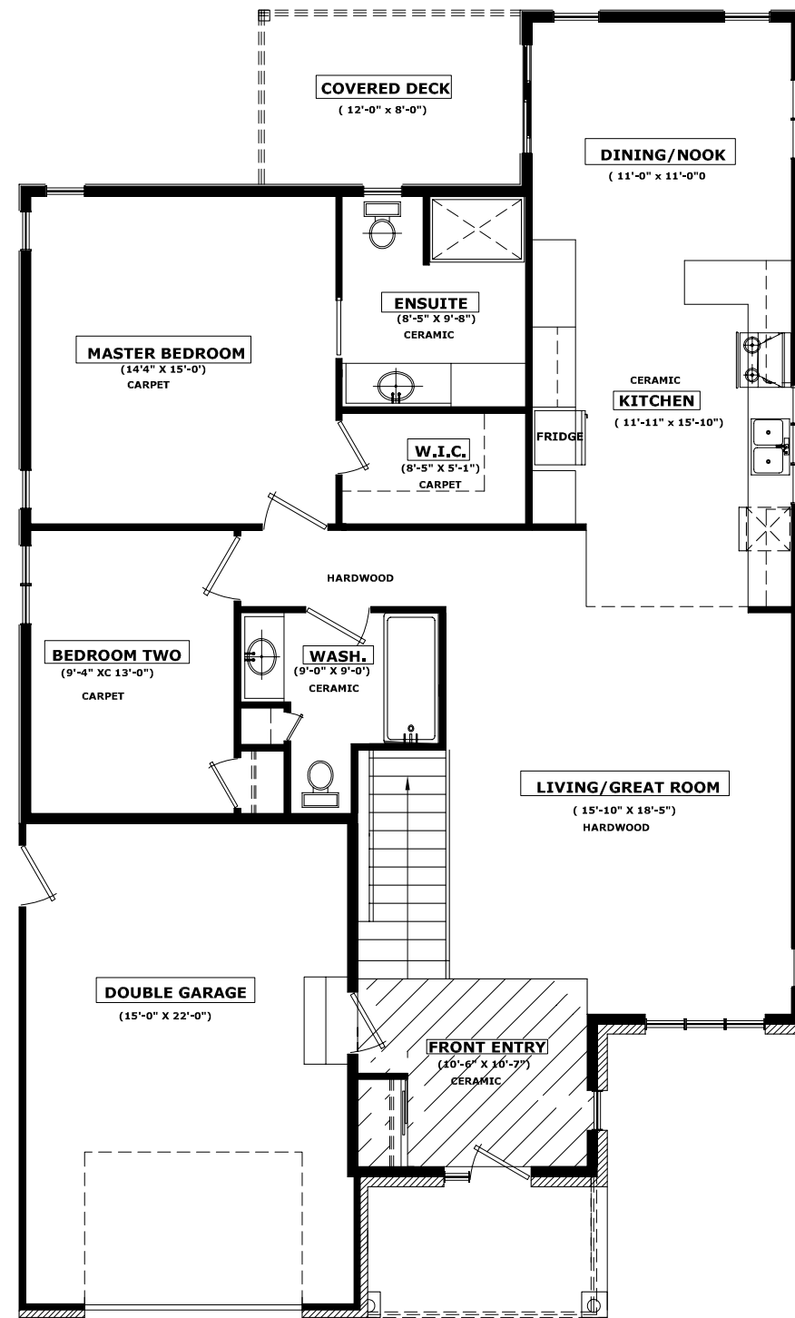
GROUND FLOOR PLAN P2901 1423 SQSFT
