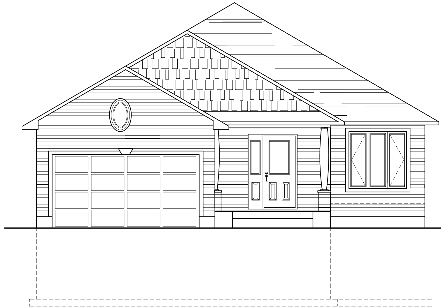
FRONT ELEVATION MODEL SAPPHIRE III 1424 SQFT
