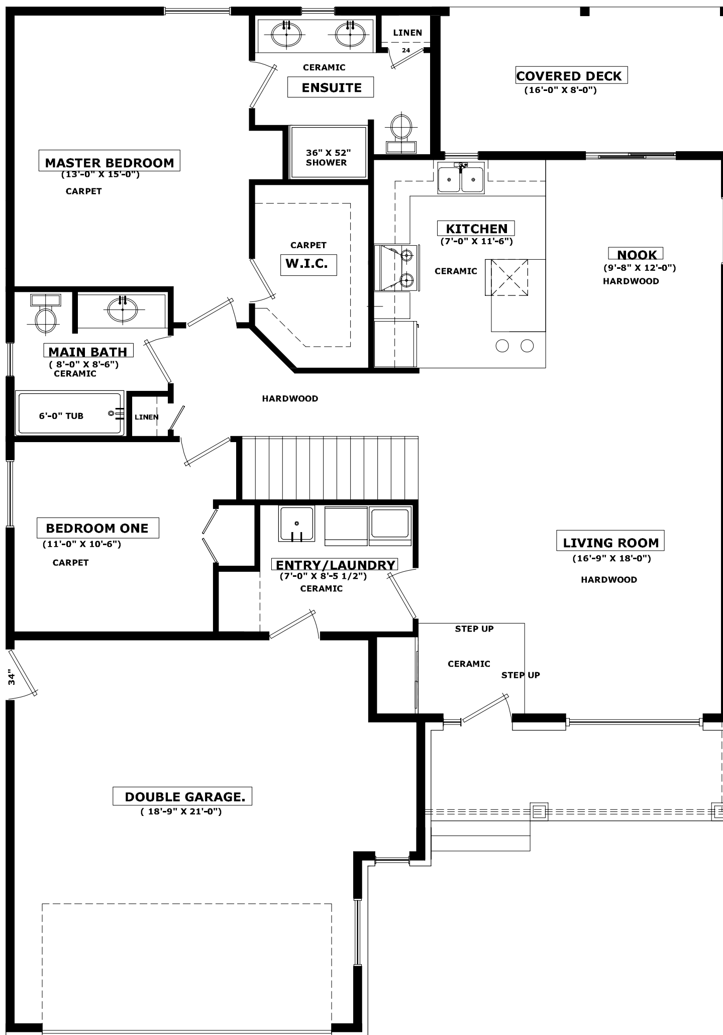
GROUND FLOOR PLAN MODEL QUARTZ 1348 SQFT
