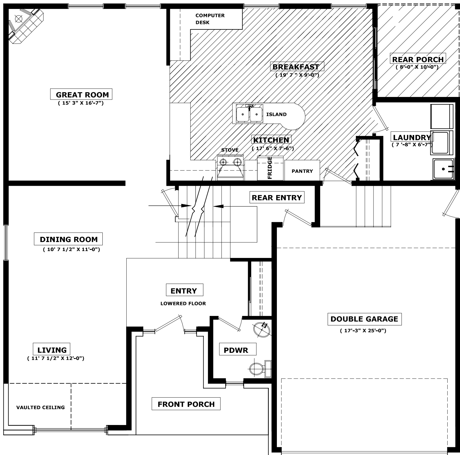
GROUND FLOOR PLAN MODEL PERIDOT 1248 SQFT.
