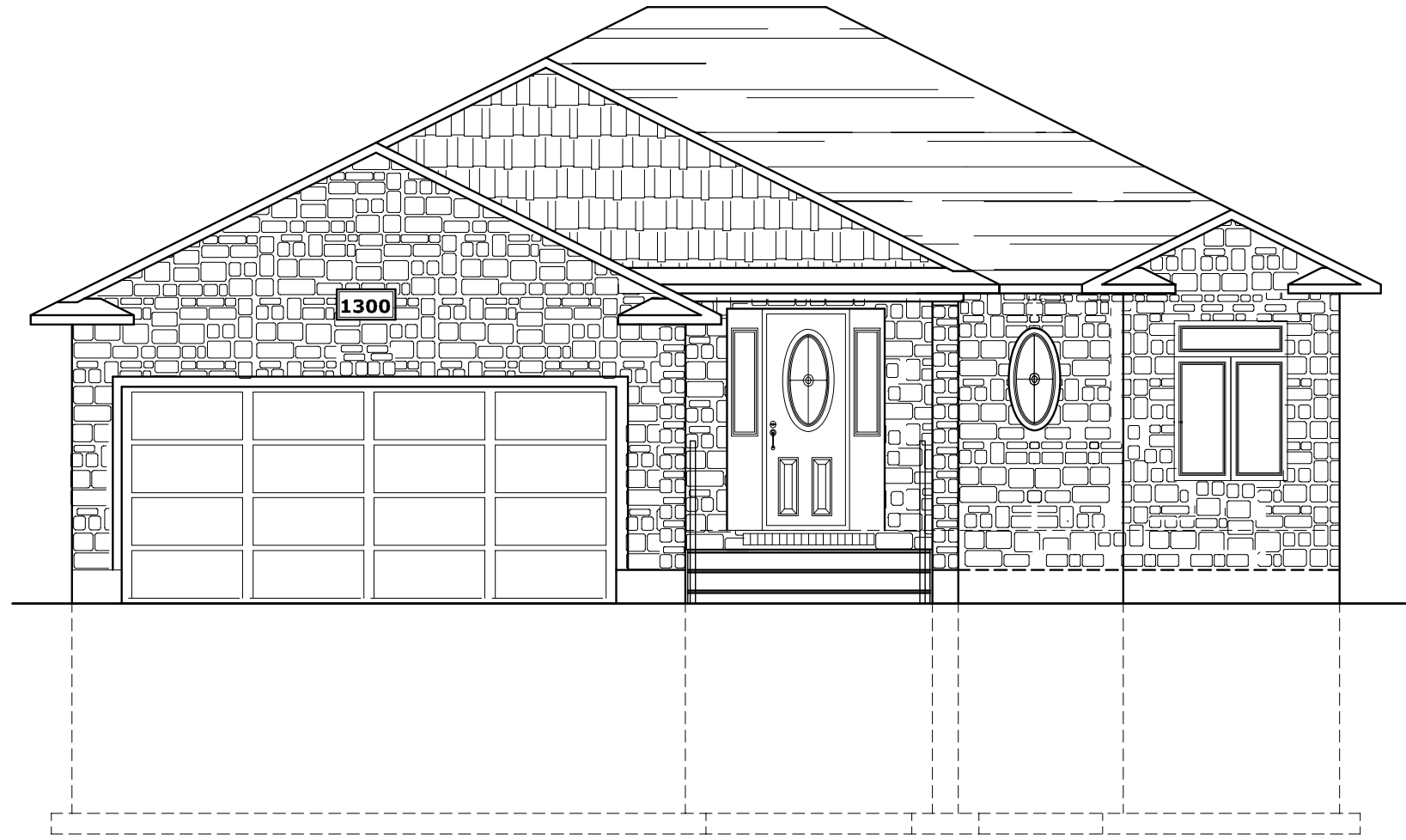
MODEL 2916 FRONT ELEVATION 1450 SQFT
