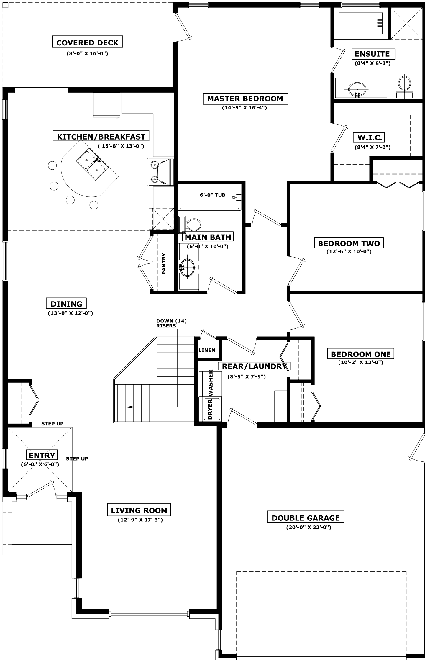
GROUND FLOOR PLAN MODEL JASPER
