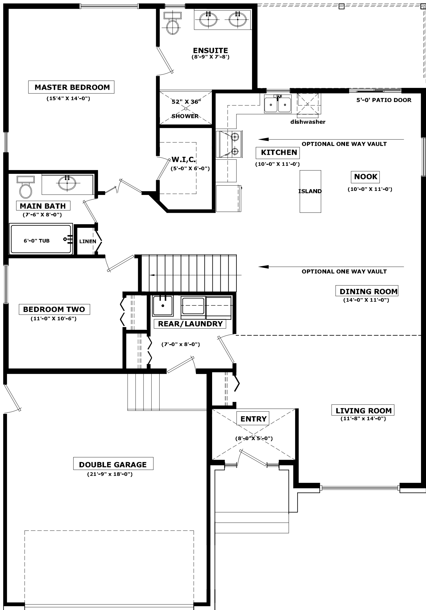
GROUND FLOOR PLAN MODEL CRYSTAL 1480 SQFT
