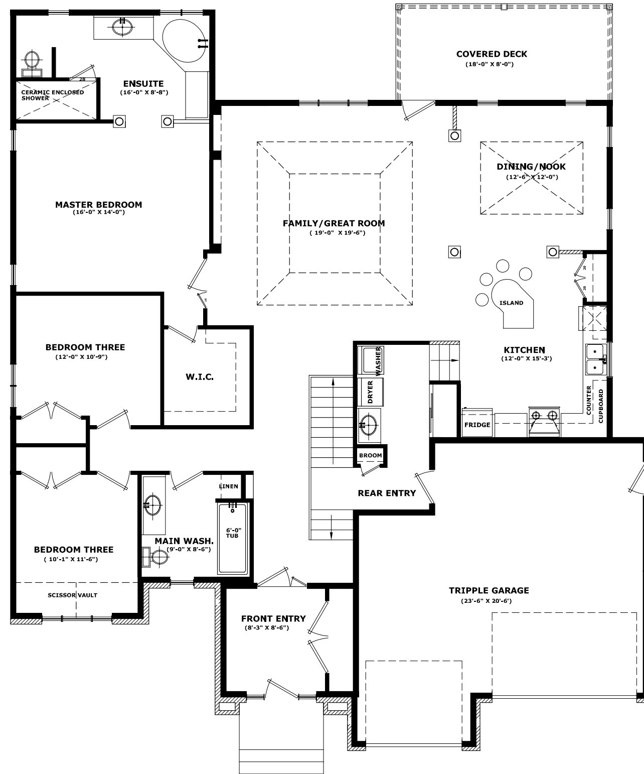
GROUND FLOOR PLAN MODEL CORALL II 2066 SQFT
