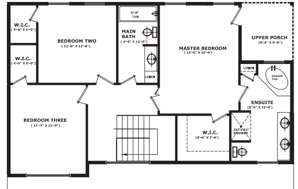
Alternate Second Floor Plan—1,052 Sq. Ft.
